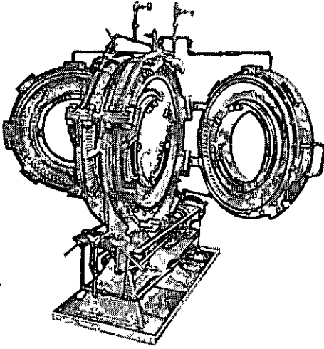
AUTOMATIC SELF-RIMMING VULCANIZER FOR TIRES AND TUBES
