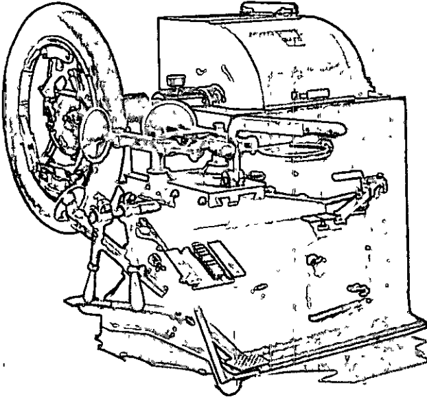
Banner Cord Tire Building Machine
