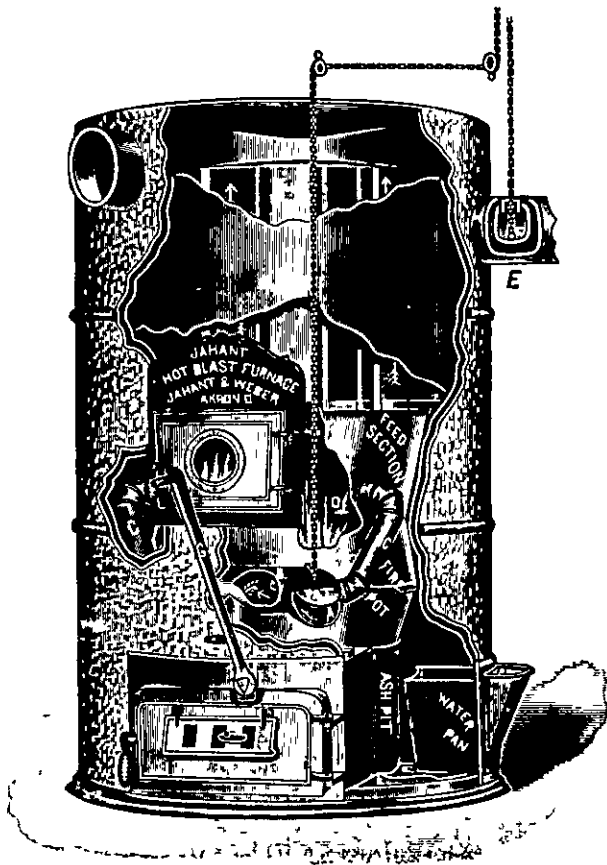
A , Air Inlet, B , Chamber in which the Air is Heated, C , Air Pipe in Hot Air Chamber, D Air Pipe in Combustion Chamber, E Check, F Dust Damper, G Shaker We Manufacture the Furnace in Five Sizes,
