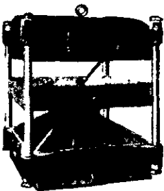
48x48 Falls Vulcanizing Press
